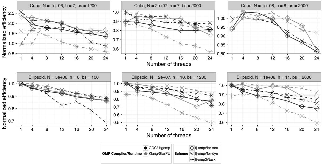
Fig. 8: Parallel efficiency normalized by the GCC/LIBGOMP fj-omp3#for-dyn sequential reference for the cube distribution (volume), above, and the ellipse (surface), below, on the 24C machine. The different plots do not use the same scale for the Normalized efficiency axis. For the largest cases (row 2, col 2–3), the fj-omp3#task scheme does not run to completion, due to the overwhelming amount of tasks being created.
