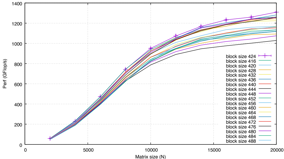
POTRF - Chameleon+StarPU, KNL-7250 1.4GHz, 16GB MCDRAM (quad,flat)
