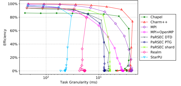
(b) 65536 bytes per task dependency.
