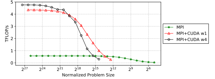
Figure 13: GPU FLOP/s vs normalized problem size (stencil, 1 node). Higher is better.
