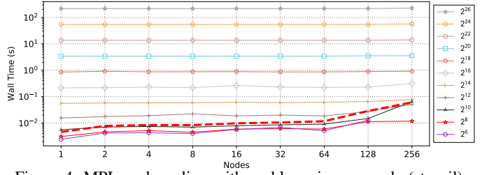
Figure 4: MPI weak scaling with problem size per node (stencil).
