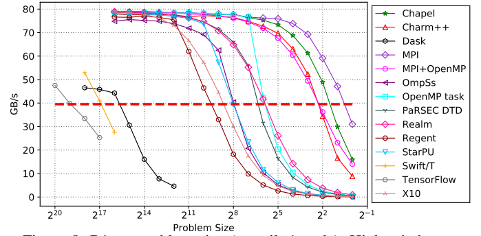
Figure 8: B/s vs problem size (stencil, 1 node). Higher is better.
