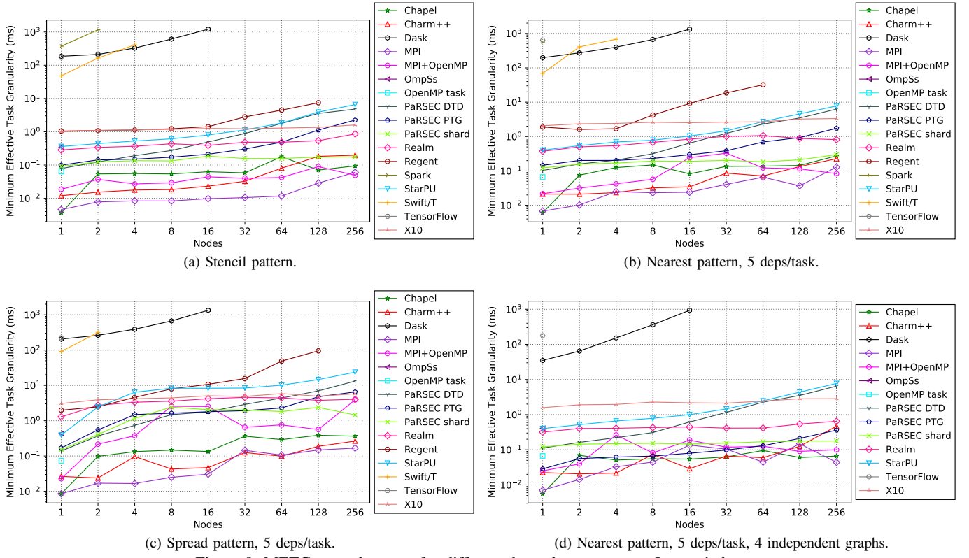
Figure 9: METG vs node count for different dependence patterns. Lower is better.
