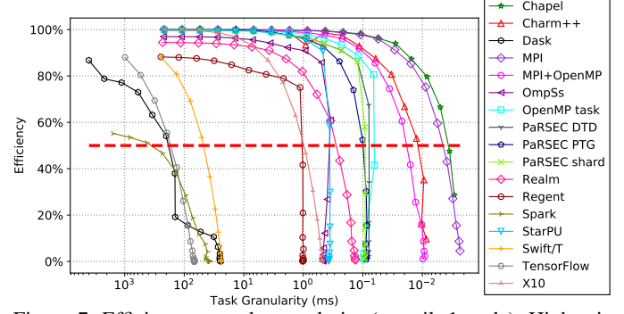
Figure 7: Efficiency vs task granularity (stencil, 1 node). Higher is better.
